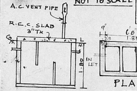
SECTION (1:50) (SEPTIC TANK)
