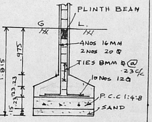
FOUNDATION DETAILS 9'x18" R.C.C. COLUMN
