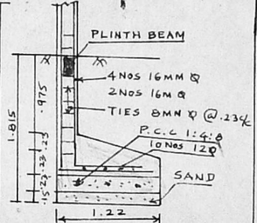
FOUNDATION DETAILS R.C.C. (9'x18") COLUMN
